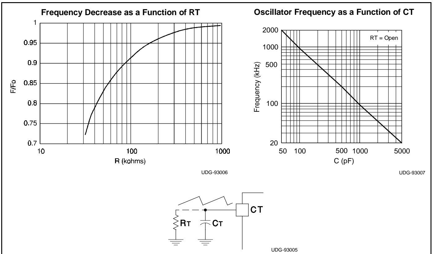
Figure 2: Oscillator Frequency
